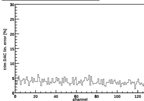
Chip Z36459A-W06-X13-Y11 trim DAC lin. error
