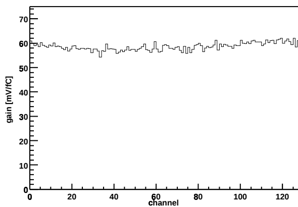
Chip Z36459A-W06-X13-Y11 Gain vs. channel
