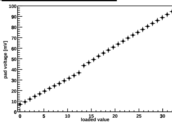
Chip Z36459A-W06-X13-Y11 preamp DAC
