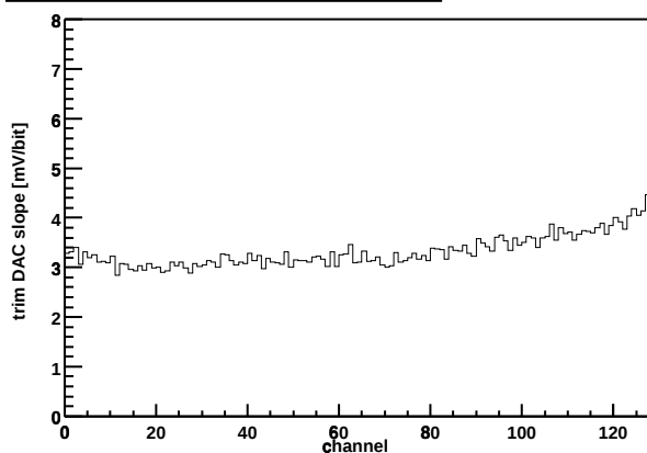
Chip Z36459A-W06-X13-Y11 Trim DAC slope vs. channel
