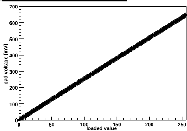
Chip Z36459A-W06-X13-Y11 threshold DAC
