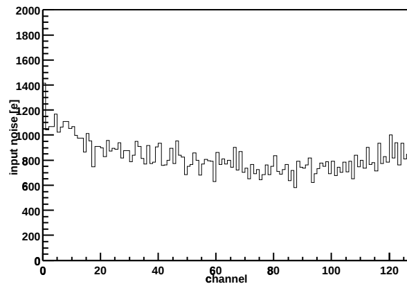
Chip Z36459A-W06-X13-Y11 Input noise vs. channel
