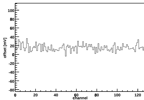
Chip Z36459A-W06-X13-Y11 Offset vs. channel
