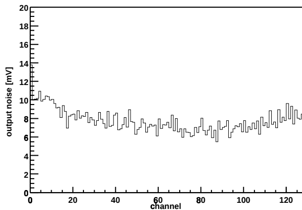
Chip Z36459A-W06-X13-Y11 Output noise vs. channel
