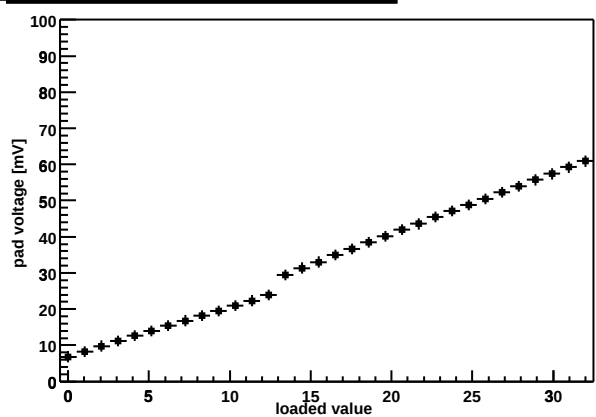
Chip Z36459A-W06-X13-Y11 shaper DAC
