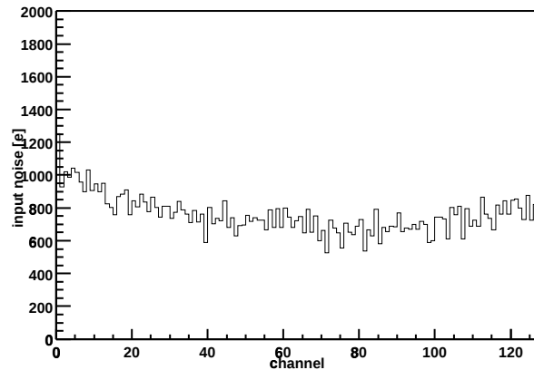
Chip Z36459A-W06-X13-Y14 Input noise vs. channel
