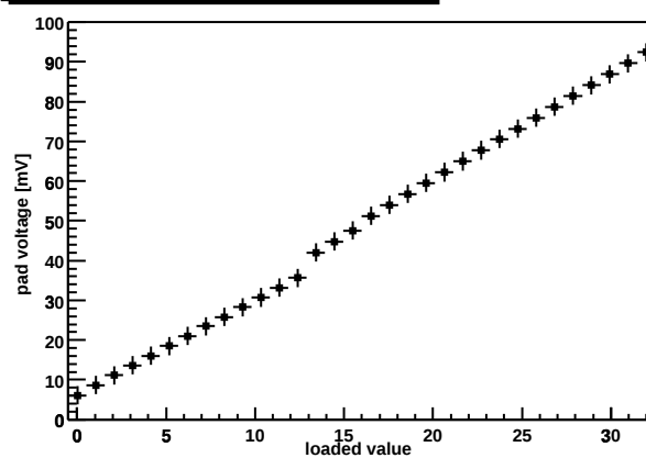
Chip Z36459A-W06-X13-Y14 preamp DAC
