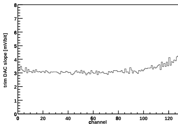
Chip Z36459A-W06-X13-Y14 Trim DAC slope vs. channel
