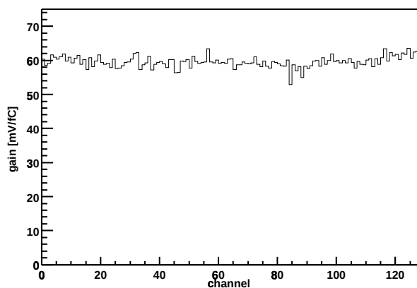
Chip Z36459A-W06-X13-Y14 Gain vs. channel
