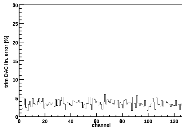
Chip Z36459A-W06-X13-Y14 trim DAC lin. error
