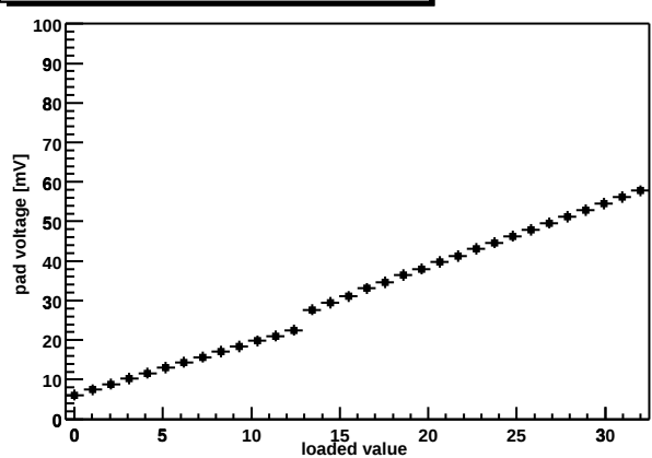
Chip Z36459A-W06-X13-Y14 shaper DAC
