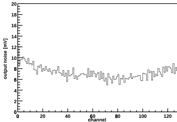
Chip Z36459A-W06-X13-Y14 Output noise vs. channel
