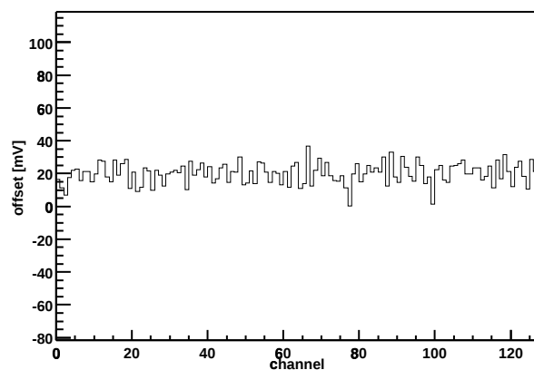
Chip Z36459A-W06-X13-Y14 Offset vs. channel
