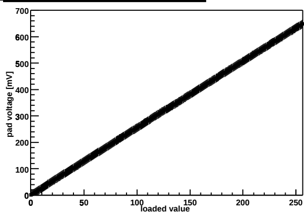
Chip Z36459A-W06-X13-Y14 threshold DAC
