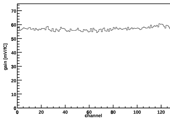
Chip Z36459A-W06-X13-Y15 Gain vs. channel
