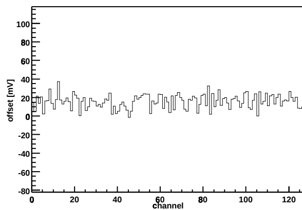
Chip Z36459A-W06-X13-Y15 Offset vs. channel
