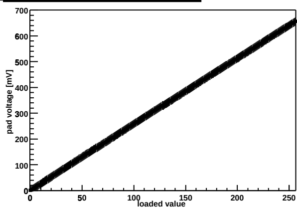
Chip Z36459A-W06-X13-Y15 threshold DAC
