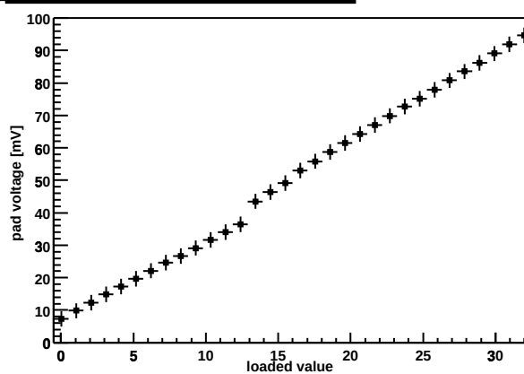
Chip Z36459A-W06-X13-Y15 preamp DAC
