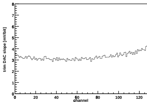
Chip Z36459A-W06-X13-Y15 Trim DAC slope vs. channel
