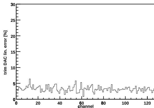
Chip Z36459A-W06-X13-Y15 trim DAC lin. error
