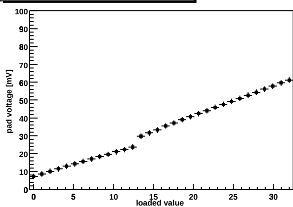
Chip Z36459A-W06-X13-Y15 shaper DAC
