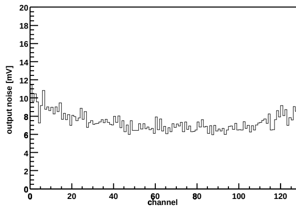
Chip Z36459A-W06-X13-Y15 Output noise vs. channel
