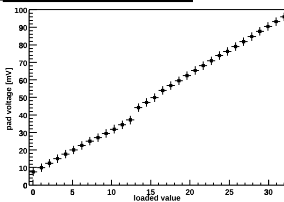
Chip Z36459A-W06-X13-Y17 preamp DAC
