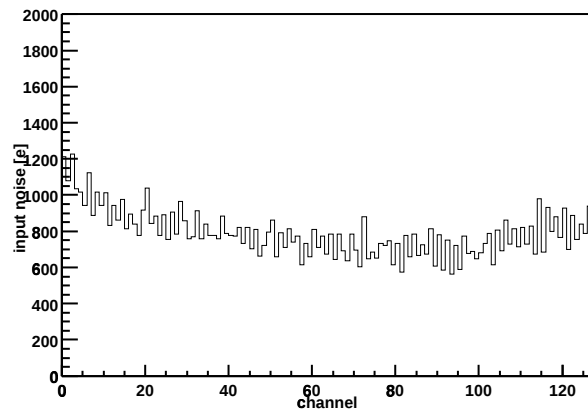
Chip Z36459A-W06-X13-Y17 Input noise vs. channel
