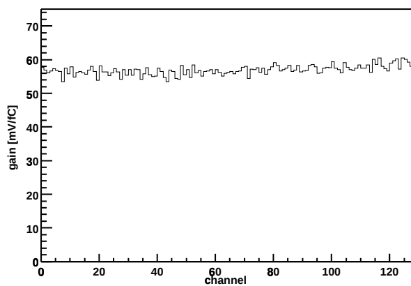
Chip Z36459A-W06-X13-Y17 Gain vs. channel
