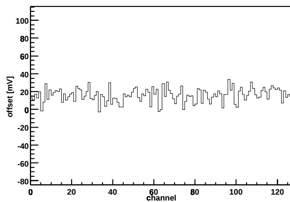
Chip Z36459A-W06-X13-Y17 Offset vs. channel
