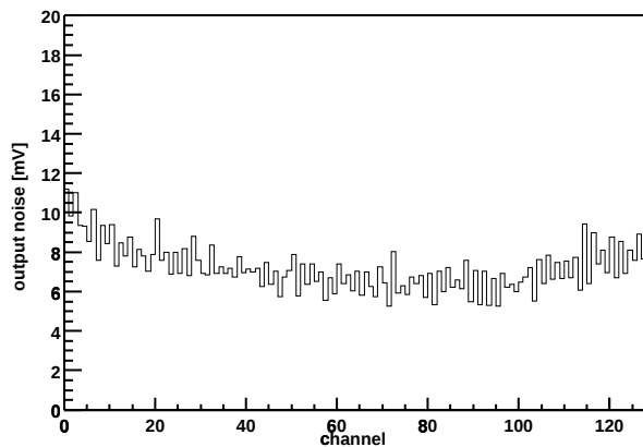
Chip Z36459A-W06-X13-Y17 Output noise vs. channel
