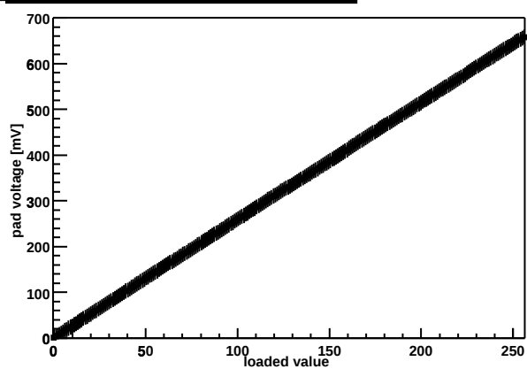
Chip Z36459A-W06-X13-Y17 threshold DAC
