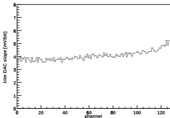
Chip Z36459A-W06-X13-Y17 Trim DAC slope vs. channel
