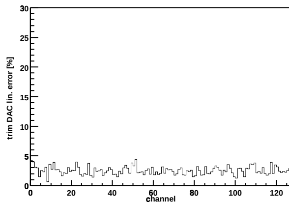
Chip Z36459A-W06-X13-Y17 trim DAC lin. error
