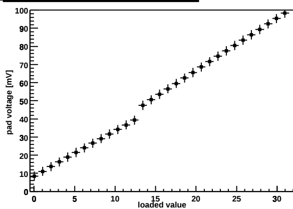
Chip Z36459A-W06-X14-Y09 preamp DAC
