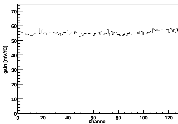
Chip Z36459A-W06-X14-Y09 Gain vs. channel
