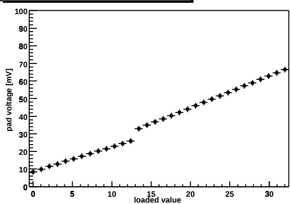
Chip Z36459A-W06-X14-Y09 shaper DAC
