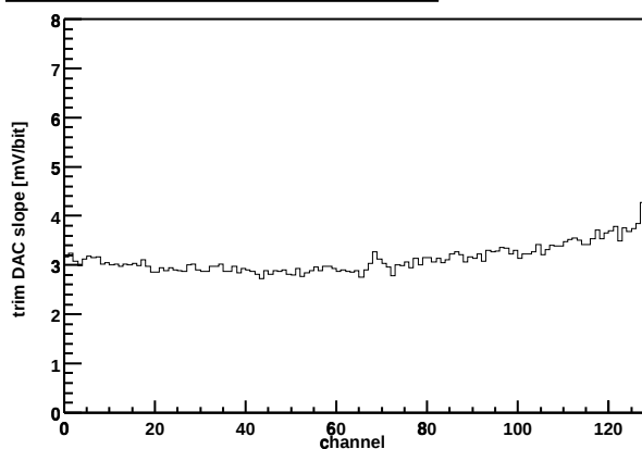
Chip Z36459A-W06-X14-Y09 Trim DAC slope vs. channel
