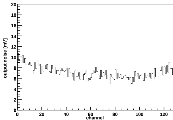
Chip Z36459A-W06-X14-Y09 Output noise vs. channel
