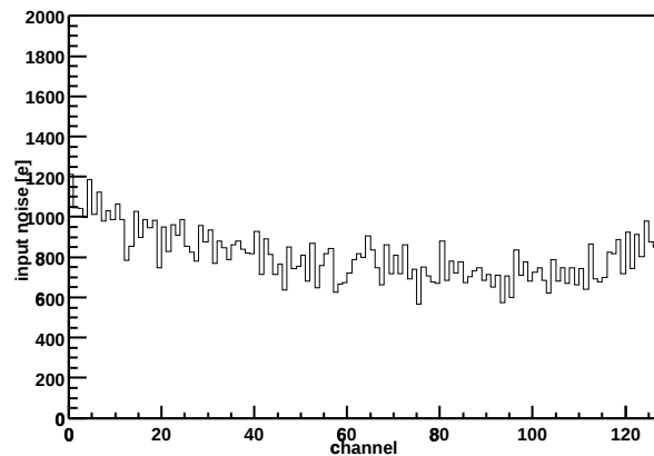
Chip Z36459A-W06-X14-Y09 Input noise vs. channel
