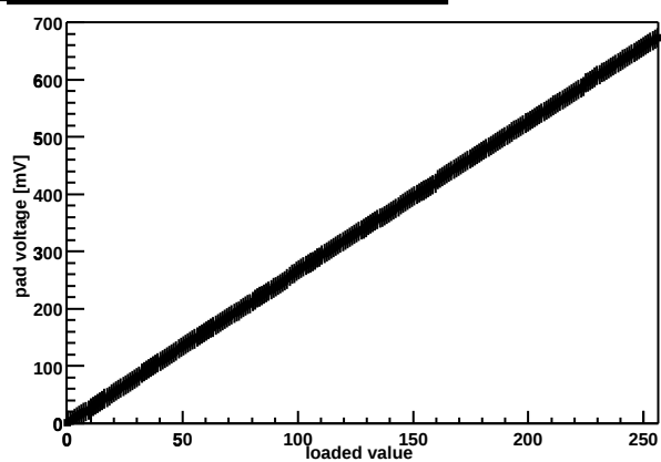
Chip Z36459A-W06-X14-Y09 threshold DAC
