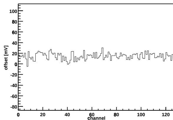
Chip Z36459A-W06-X14-Y14 Offset vs. channel
