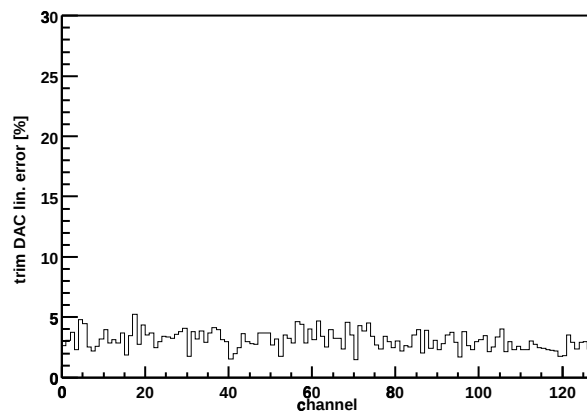
Chip Z36459A-W06-X14-Y14 trim DAC lin. error
