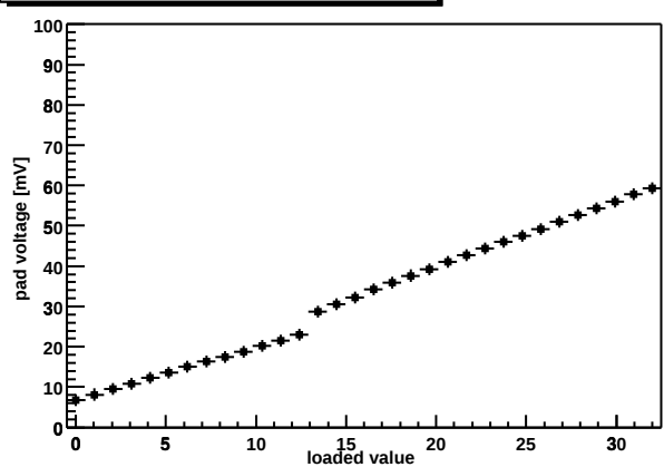
Chip Z36459A-W06-X14-Y14 shaper DAC
