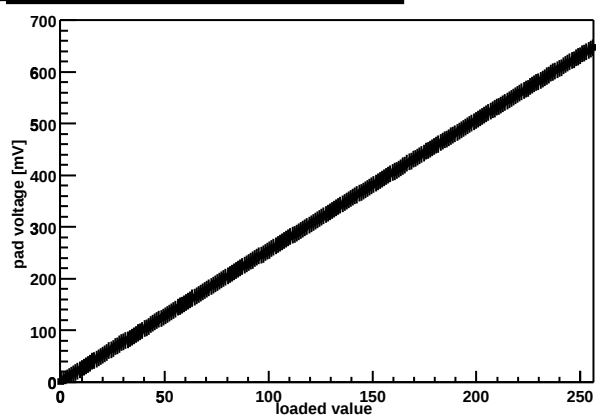
Chip Z36459A-W06-X14-Y14 threshold DAC
