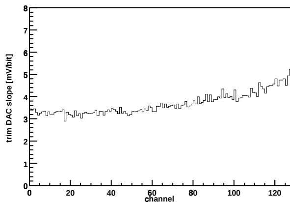
Chip Z36459A-W06-X14-Y14 Trim DAC slope vs. channel
