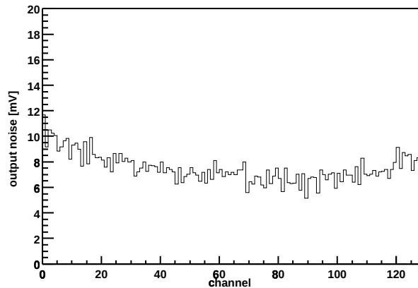
Chip Z36459A-W06-X14-Y14 Output noise vs. channel
