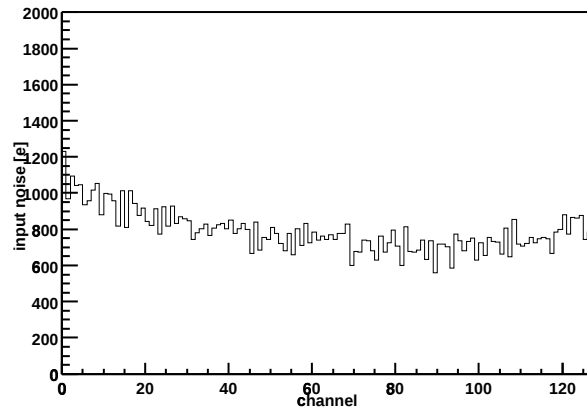
Chip Z36459A-W06-X14-Y14 Input noise vs. channel
