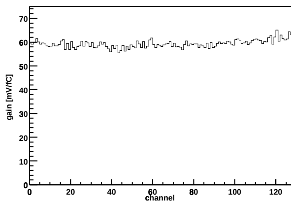
Chip Z36459A-W06-X14-Y14 Gain vs. channel
