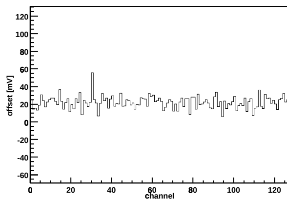
Chip Z36459A-W06-X14-Y17 Offset vs. channel
