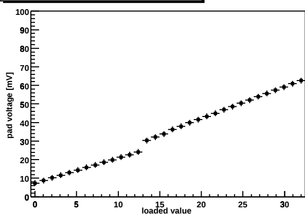
Chip Z36459A-W06-X14-Y17 shaper DAC
