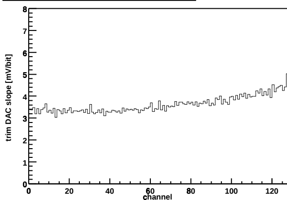
Chip Z36459A-W06-X14-Y17 Trim DAC slope vs. channel
