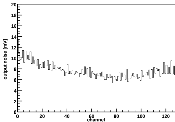
Chip Z36459A-W06-X14-Y17 Output noise vs. channel
