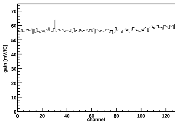
Chip Z36459A-W06-X14-Y17 Gain vs. channel
