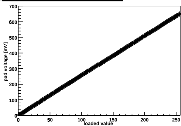
Chip Z36459A-W06-X14-Y17 threshold DAC
