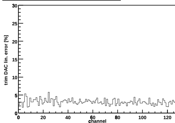
Chip Z36459A-W06-X14-Y17 trim DAC lin. error
