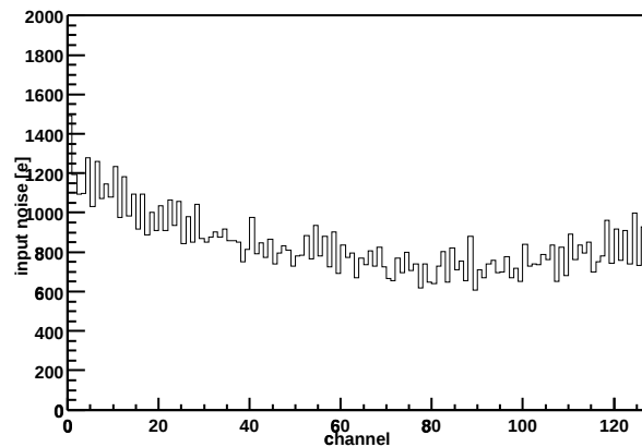
Chip Z36459A-W06-X14-Y17 Input noise vs. channel
