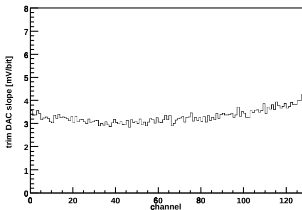
Chip Z36459A-W06-X15-Y06 Trim DAC slope vs. channel
