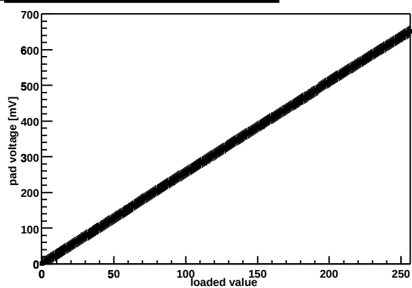
Chip Z36459A-W06-X15-Y06 threshold DAC
