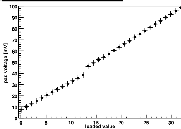
Chip Z36459A-W06-X15-Y06 preamp DAC
