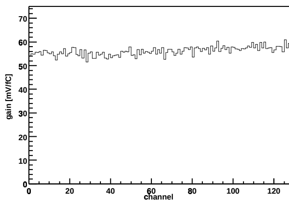
Chip Z36459A-W06-X15-Y06 Gain vs. channel
