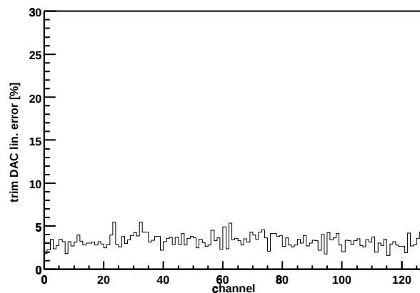
Chip Z36459A-W06-X15-Y06 trim DAC lin. error
