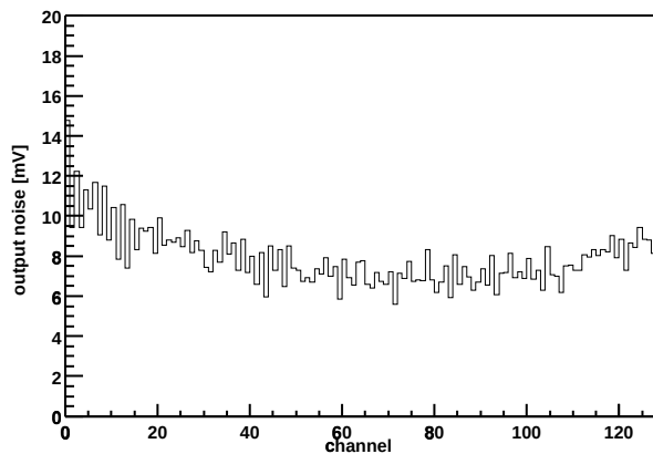
Chip Z36459A-W06-X15-Y06 Output noise vs. channel
