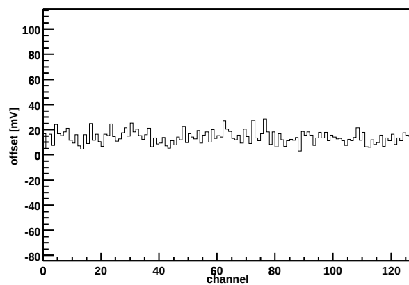
Chip Z36459A-W06-X15-Y06 Offset vs. channel
