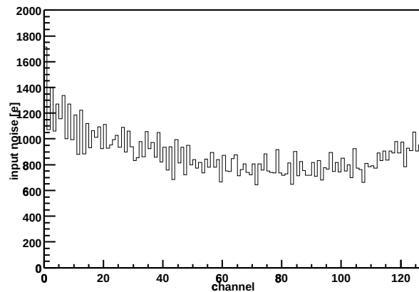
Chip Z36459A-W06-X15-Y06 Input noise vs. channel
