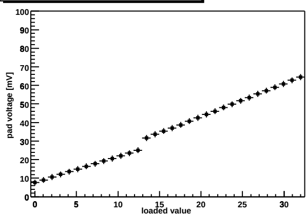
Chip Z36459A-W06-X15-Y06 shaper DAC
