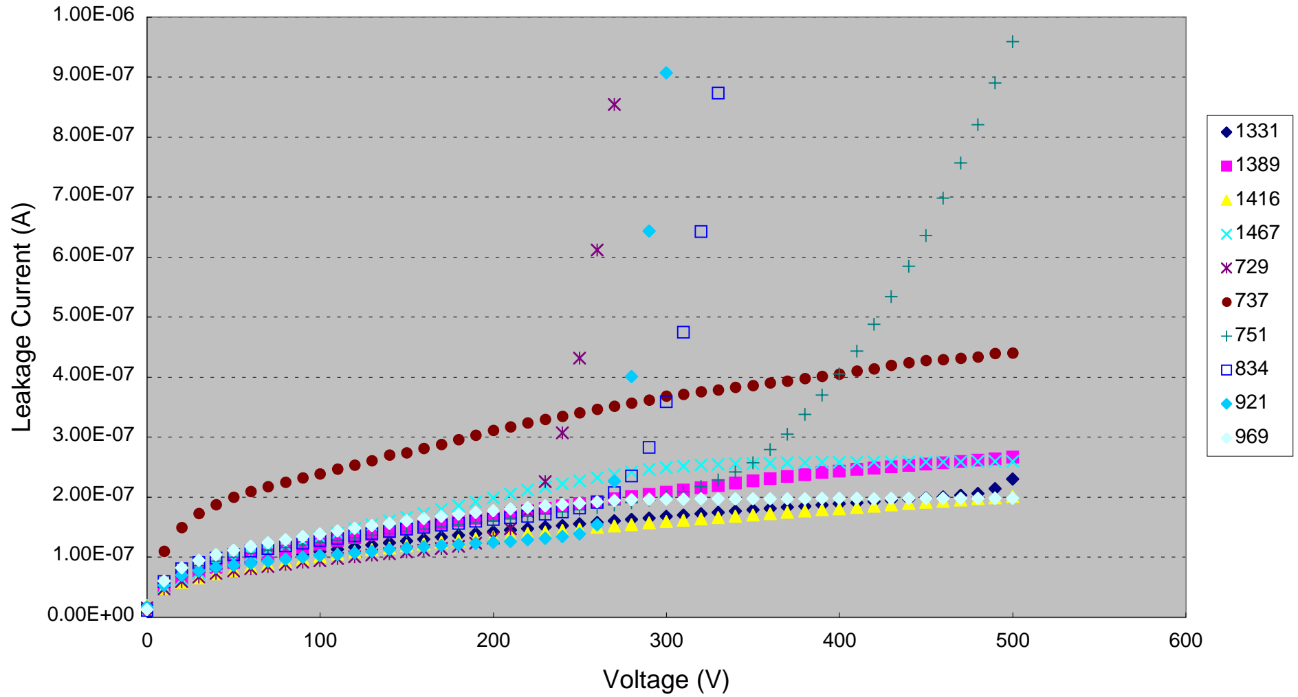
I-V Curve (Sensors for April01 irradiation)
