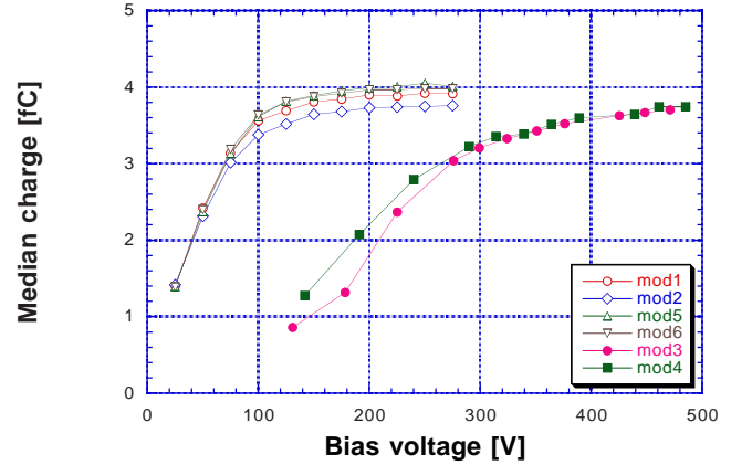
Figure 13: Bias voltage dependence of the median charges.
