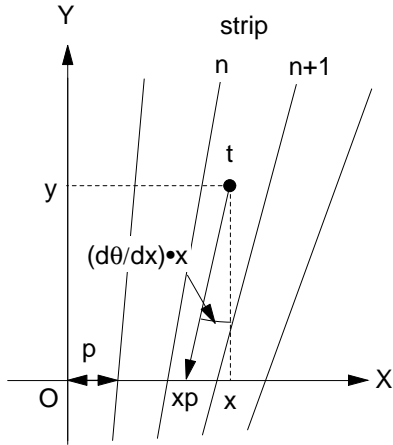
Figure 7: Correction of the fan geometry. A hit at t=(x, y) is projected at the hit x_1 at the x -axis of the pitch p , approximated as xp=x+(d\theta/dx)\cdot x\cdot y
