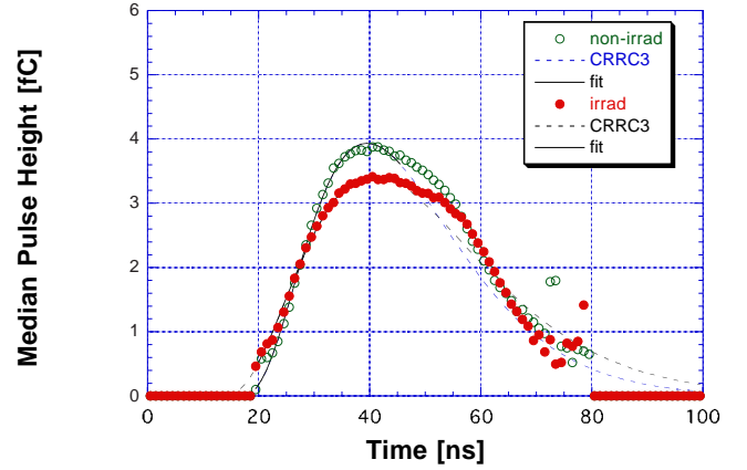
Figure 4: Median pulse height distributions as a function of time between trigger and clock phase: non-irradiated (open circle) and irradiated (filled circle) modules, and the impulse responses of CR-RC 3 circuitry (solid line being the fitted region) with the peaking times of 22 and 27 ns, respectively
