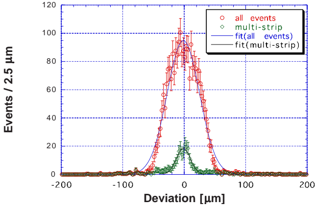
Figure 6: Deviations of the cluster centre from the expected positions of incident particles of the mod1 module: all events (circles) and the events with multi-hits (diamonds), with Gaussian fits without weighting
