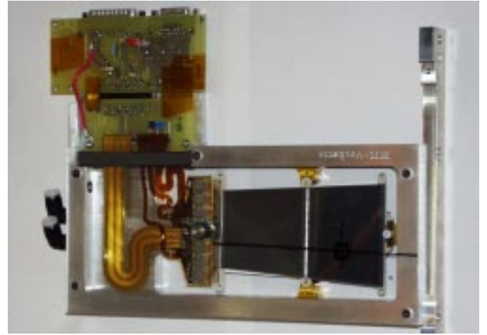
Figure 2: ATLAS SCT endcap module, together with a module frame and a readout card at the beamtest
