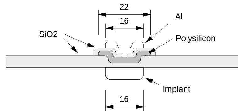
ATLAS98 wide-polysilicon
