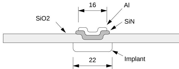
ATLAS98 baseline
