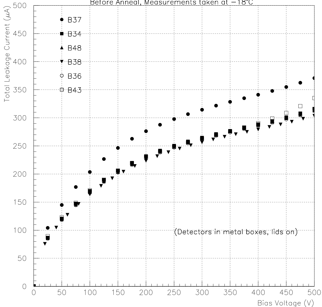
HAMAMATSU DETECTORS IRRADIATED JUNE 99 Before Anneal, Measurements taken at -18^{\circ}\text{C}
