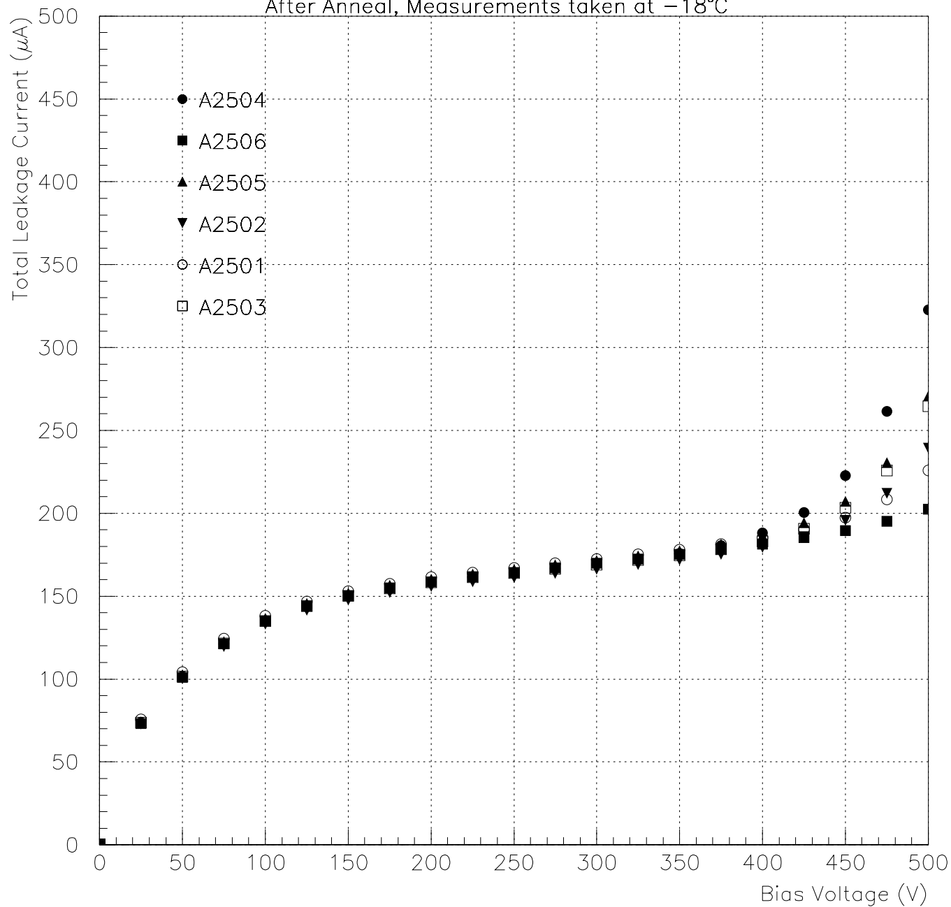
HAMAMATSU DETECTORS IRRADIATED JUNE 99 After Anneal, Measurements taken at -18^{\circ}\text{C}
