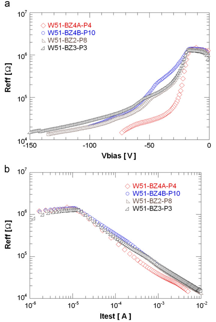
Fig. 4. DC scan of effective resistance R_{\text{eff}} as a function of (a) applied voltage and (b) current, between strip DC pad and the bias ring, respectively. One probe is used to stimulate and measure. The resistance–voltage scan is an extension to higher voltages of the data of Ref. [8], where V_{\text{PT}} \approx 20 V was found.
