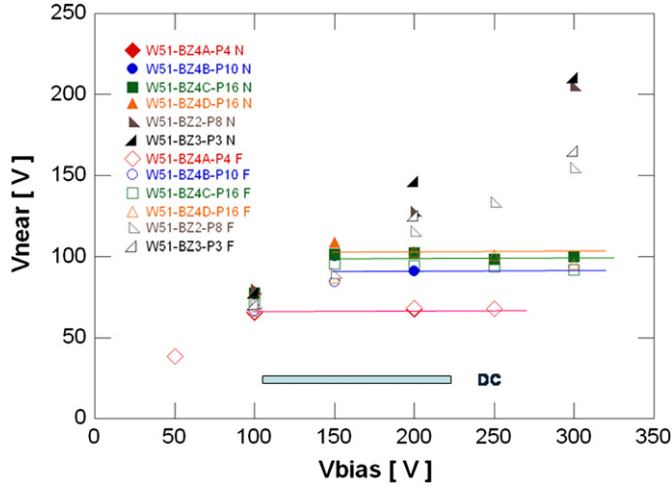
Fig. 3. Peak voltages V_{\text{near}} measured at the “near” implant location as a function of the bias voltage. The data with laser “near” injection are shown with filled symbols and the letter “N”. The data with laser “far” location are shown with open symbols and the letter “F”. The DC PT voltages, as defined in Section 3, are shown as a band.
