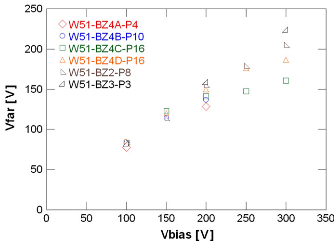
Fig. 10. Voltages V_{far} measured at the “far” implant location as a function of bias voltage. The laser pulse was injected at the “far” location as well. This should be compared with Fig. 3, where V_{near} showed saturation for the PTP structures below or at about 100 V.
