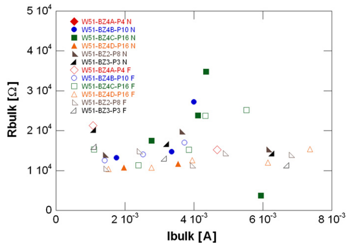
Fig. 6. Current dependence of the bulk resistance R_{bulk} for both laser positions.
