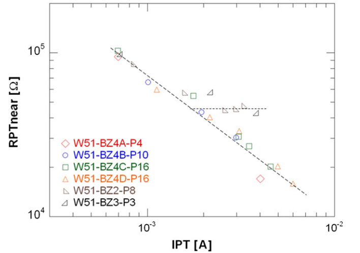
Fig. 8. Current dependence of R_{PT}(\text{near}) showing the approximate 1/i dependence and the leveling-off of the non-PTP structures BZ2 and BZ3. The lines are to guide the eye.
