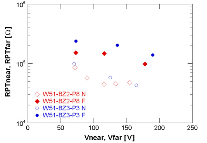
Fig. 7. Voltage dependence of the resistance R_{PT} for the structures BZ2 and BZ3 without PTP structure. Open symbols are R_{PT}(\text{near}) , filled symbols are R_{PT}(\text{far}) .
