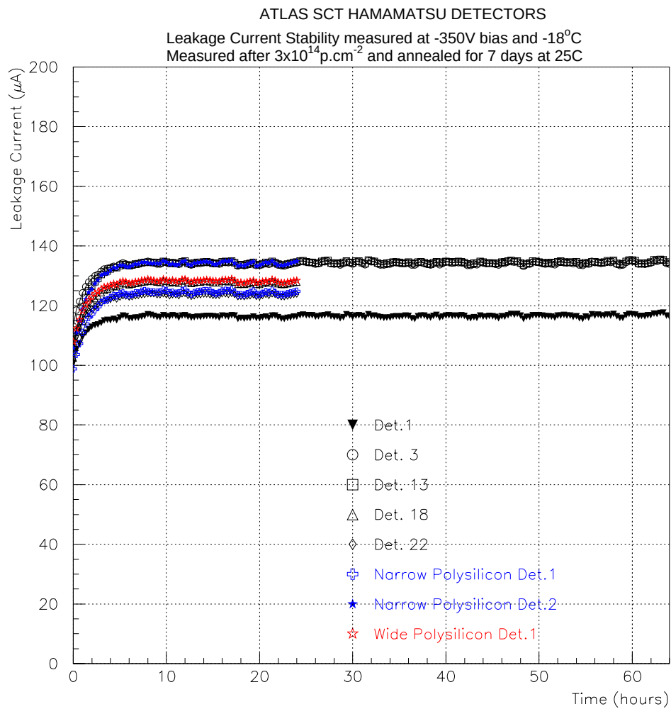
Fig. 2. Stability of the leakage current at 350V and at -18°C.
