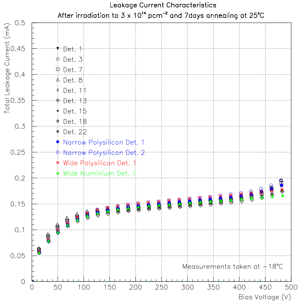
Fig. 1. Leakage current characteristics for all detector designs after irradiation and annealing.
