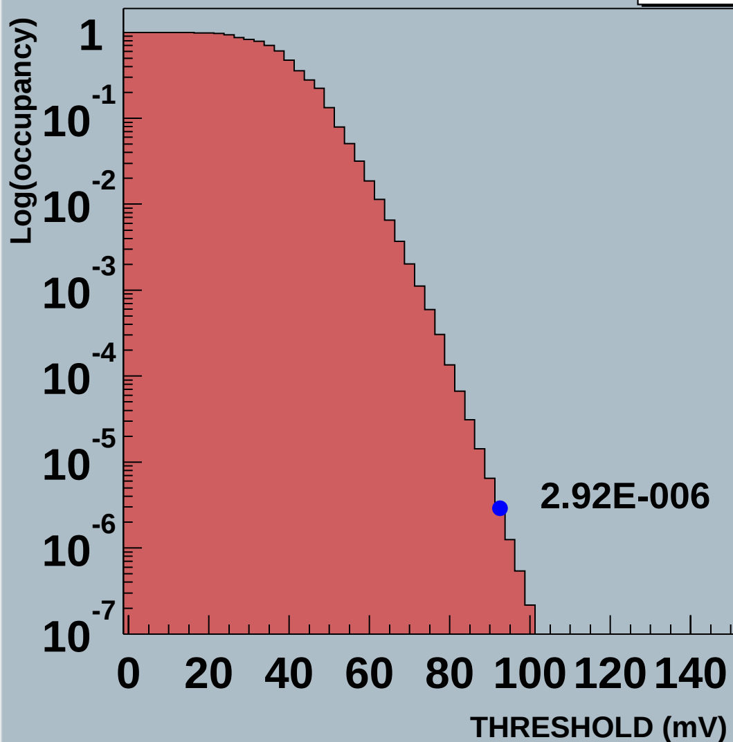
Module 3 20220170200400mDaqLTL Noise Occupancy
