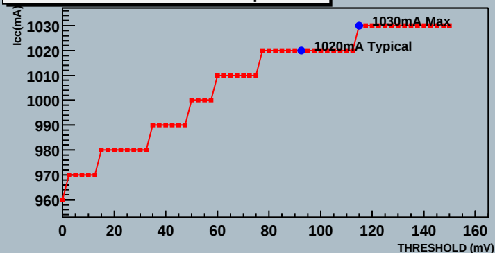
Module 3 20220170200400mDaqLTL Idd
