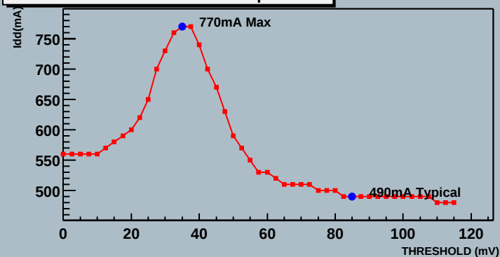
Module 2 20220170200400mDaqLT Power
