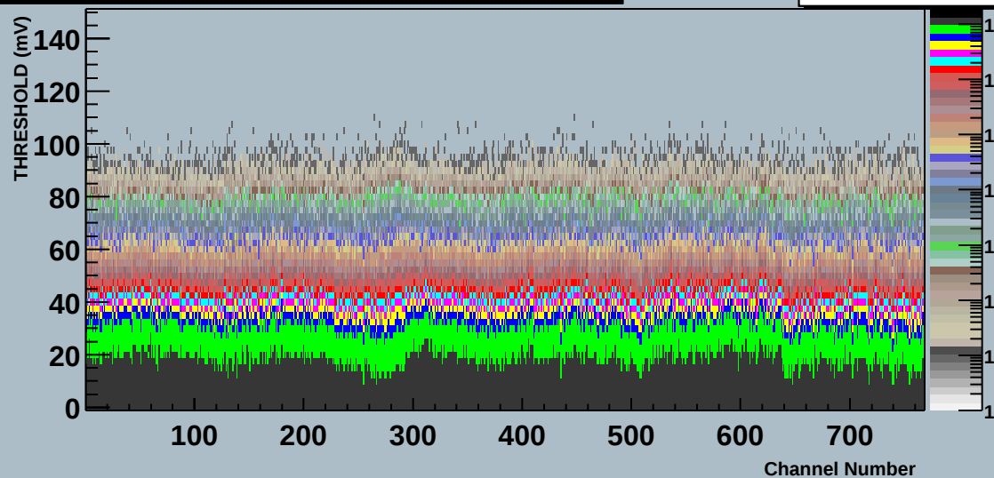
Module 2 20220170200400mDaqLT Stream 1 THRESHOLD (mV) Scan
