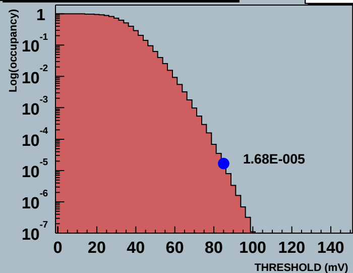
Module 2 20220170200400mDaqLT Stream 1 THRESHOLD (mV) Scan
