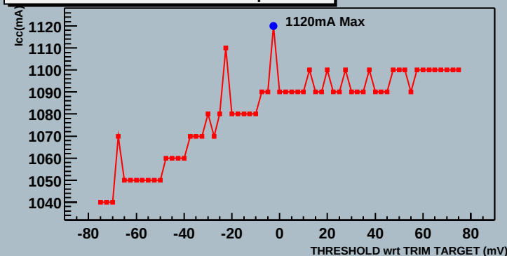
Module 1 20220170200832mDaqLTL Idd
