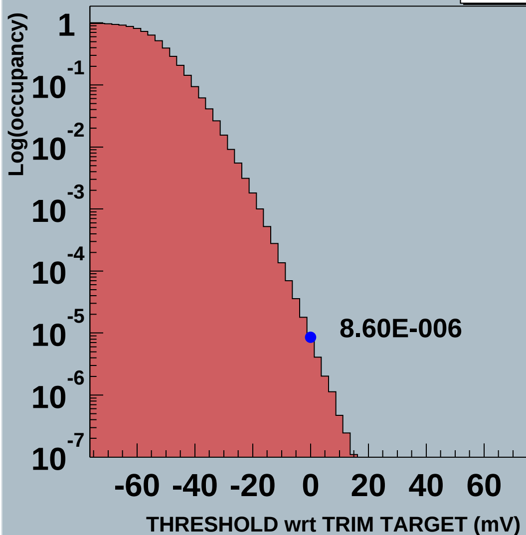
Module 1 20220170200832mDaqLTL Noise Occupancy
