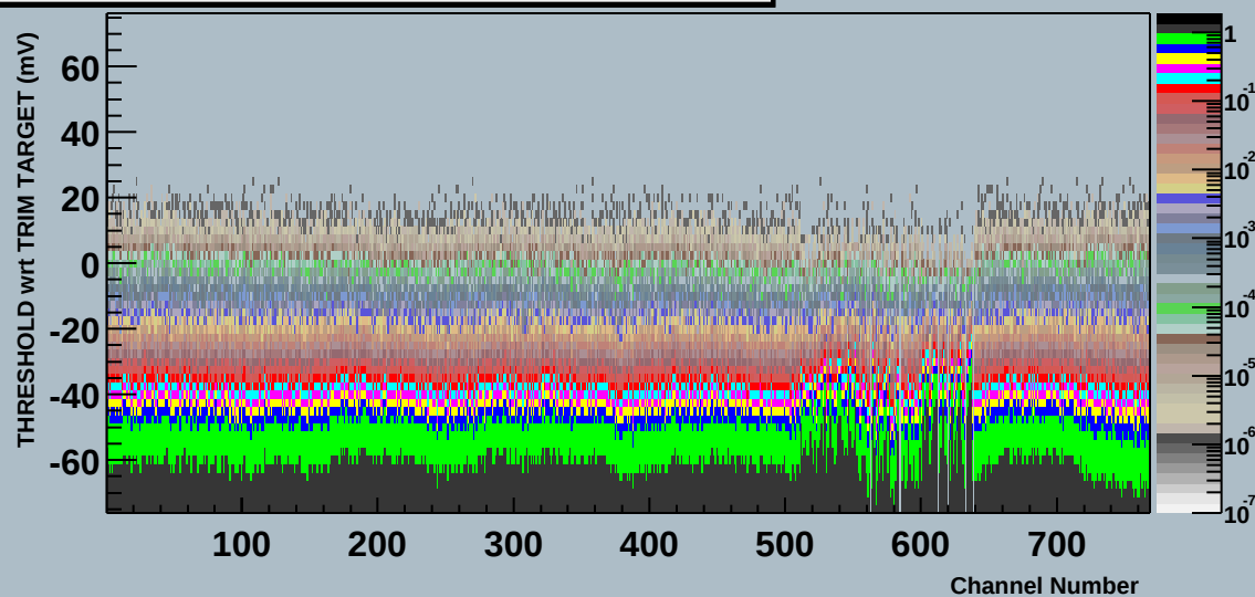
Module 0 20220170200967mDaqLT Stream 1 THRESHOLD wrt TRIM TARGET (mV) Scan
