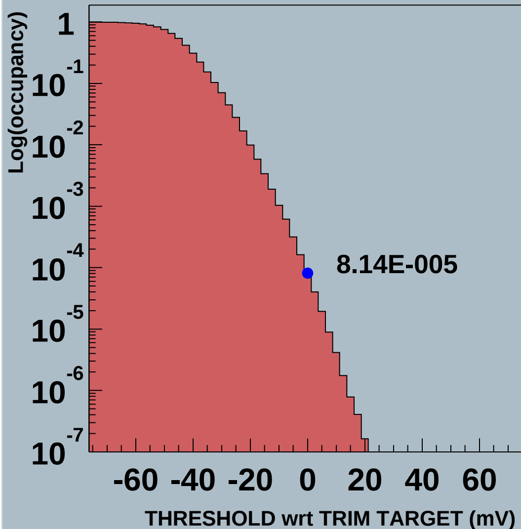
Module 0 20220170200967mDaqLT Noise Occupancy
