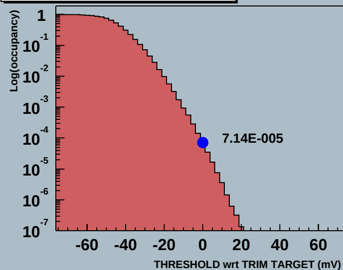
Module 0 20220170200967mDaqLT Stream 1 THRESHOLD wrt TRIM TARGET (mV) Scan
