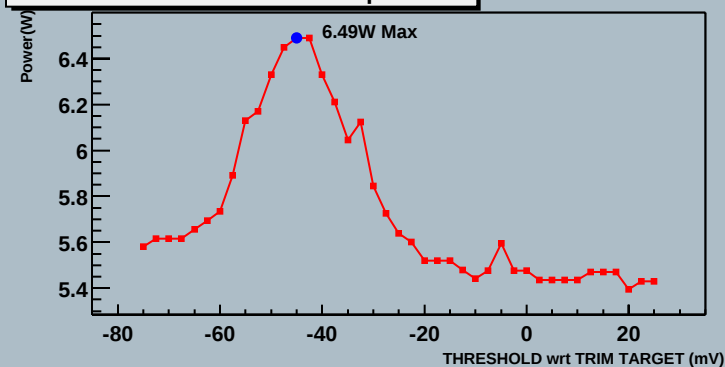
Module 0 20220170200967mDaqLT Power
