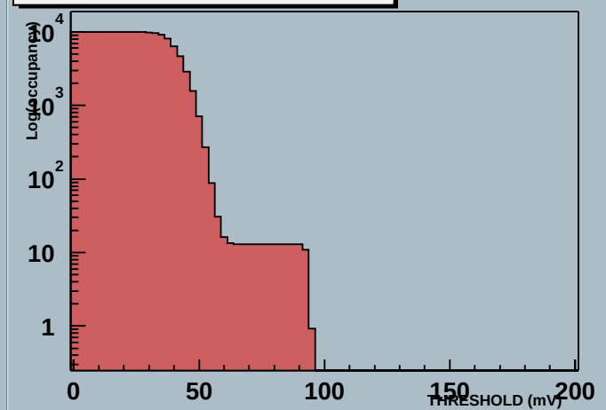
Module 0 60000000000598hDaqIN Stream 1 THRESHOLD (mV) Scan
