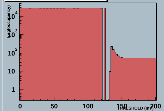
Module 0 60000000000622hDaqPR Stream 1 THRESHOLD (mV) Scan
