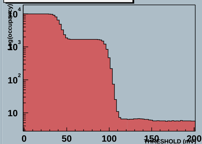
Module 1 60000000000628hDaqIN Stream 1 THRESHOLD (mV) Scan
