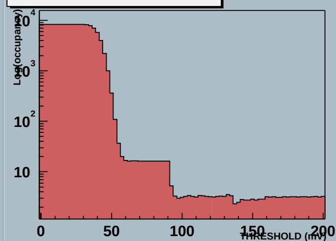
Module 5 60000000000618hDaqIN Stream 1 THRESHOLD (mV) Scan
