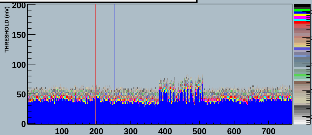
Module 0 60000000000627hDaqIN Stream 1 THRESHOLD (mV) Scan
