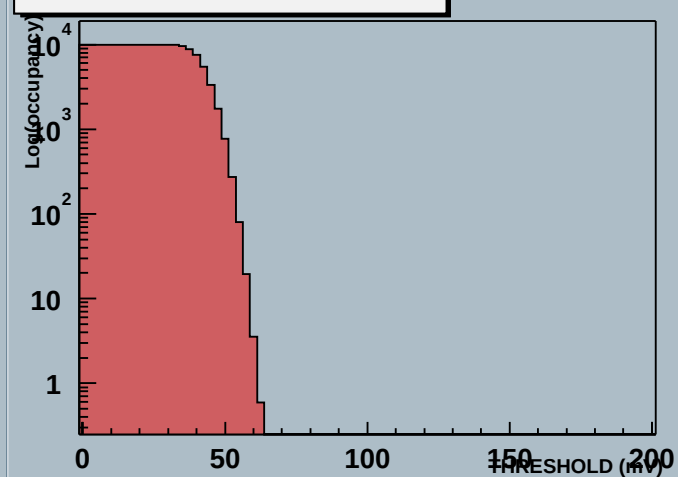
Module 5 60000000000618hDaqIN Stream 1 THRESHOLD (mV) Scan
