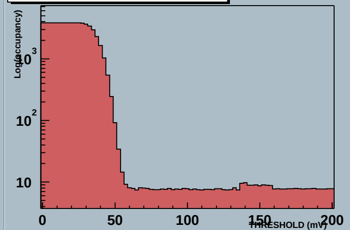
Module 0 60000000000598hDaqIN Stream 1 THRESHOLD (mV) Scan
