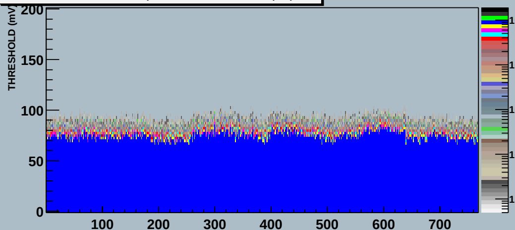
Module 2 60000000000629hDaqIN Stream 1 THRESHOLD (mV) Scan
