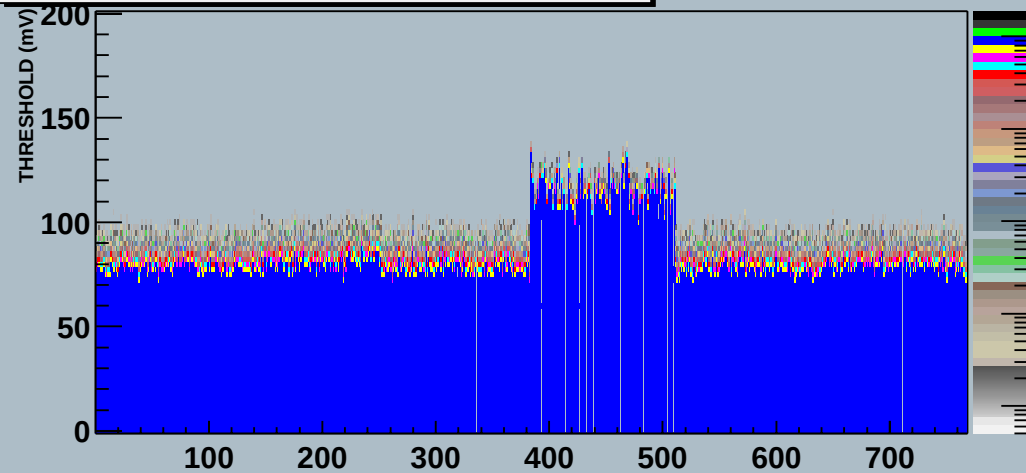
Module 0 60000000000623hDaqIN Stream 1 THRESHOLD (mV) Scan
