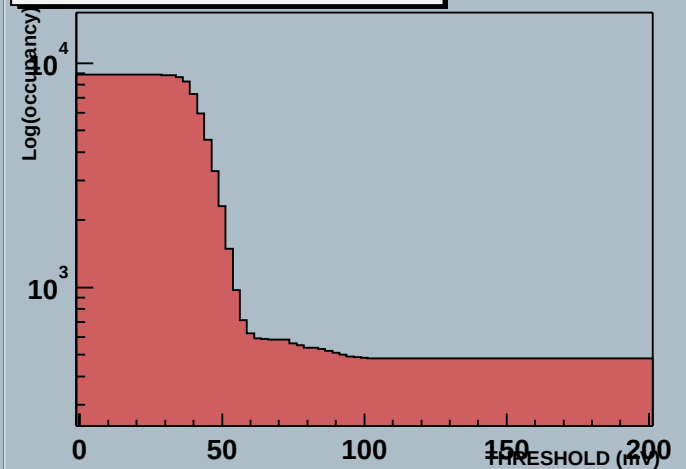
Module 2 60000000000612hDaqIN Stream 1 THRESHOLD (mV) Scan
