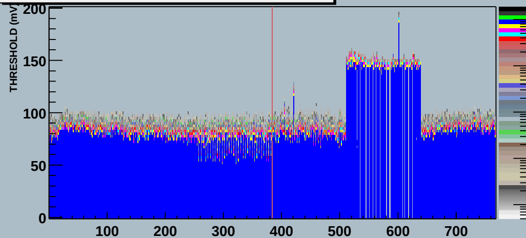
Module 0 60000000000623hDaqIN Stream 1 THRESHOLD (mV) Scan
