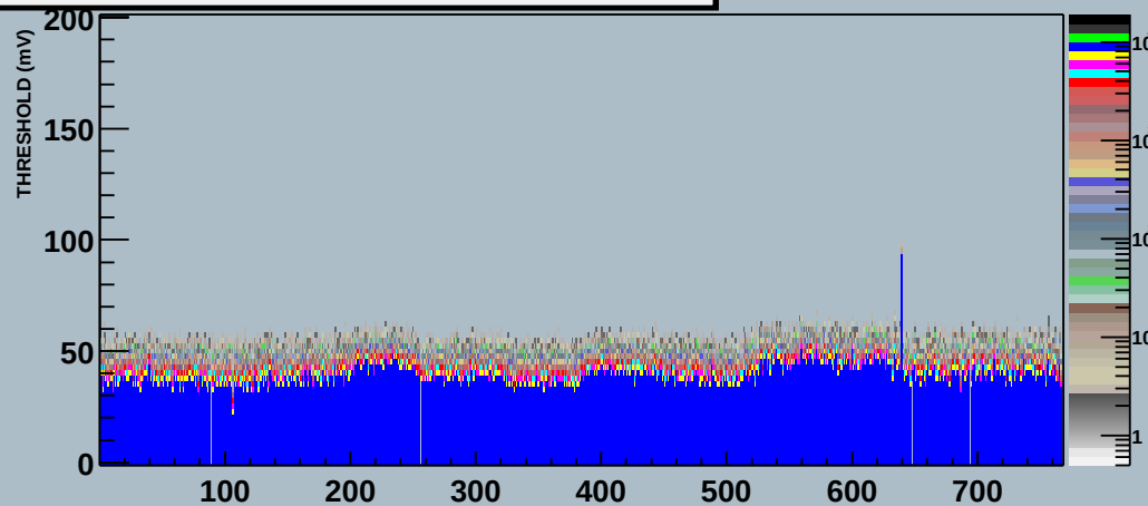
Module 0 60000000000598hDaqIN Stream 1 THRESHOLD (mV) Scan
