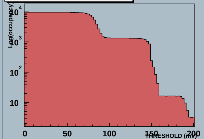
Module 0 60000000000623hDaqIN Stream 1 THRESHOLD (mV) Scan
