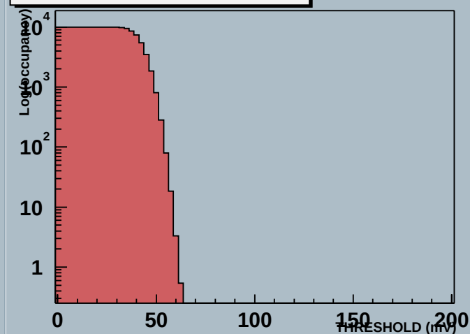
Module 2 60000000000602hDaqIN Stream 1 THRESHOLD (mV) Scan
