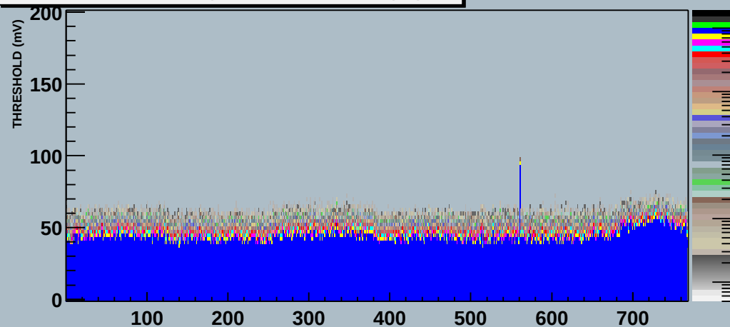
Module 0 60000000000626hDaqIN Stream 1 THRESHOLD (mV) Scan
