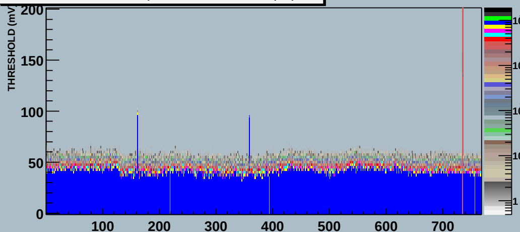
Module 2 60000000000602hDaqIN Stream 1 THRESHOLD (mV) Scan
