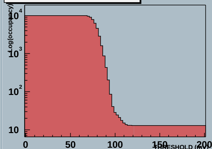
Module 3 60000000000616hDaqIN Stream 1 THRESHOLD (mV) Scan
