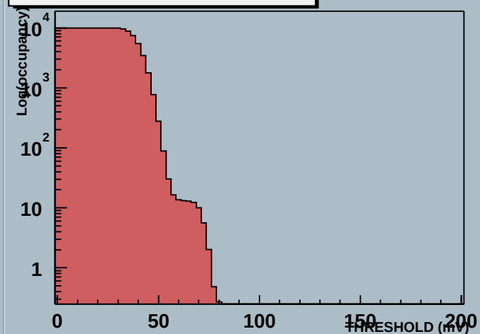
Module 1 60000000000628hDaqIN Stream 1 THRESHOLD (mV) Scan
