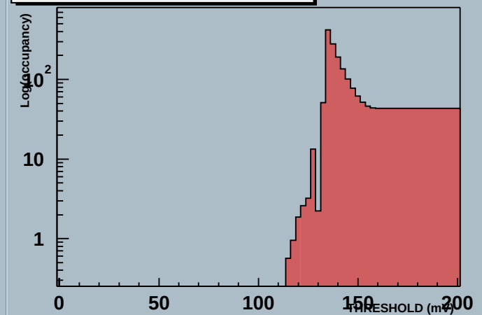
Module 0 60000000000622hDaqPR Stream 1 THRESHOLD (mV) Scan
