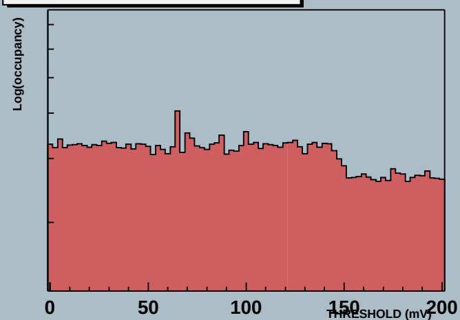
Module 0 60000000000627hDaqIN Stream 1 THRESHOLD (mV) Scan
