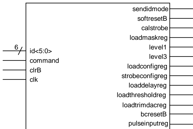
Figure 3.8B. Command Decoder Inputs/Outputs (ABCD2T).
