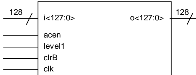
Figure 3.2. Pipeline Input/Outputs.
