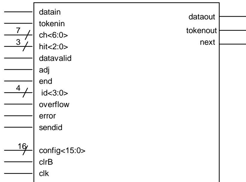
Figure 3.6. Connections to Readout Circuitry.
