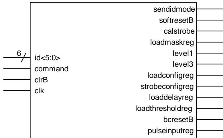
Figure 3.8A. Command Decoder Inputs/Outputs (ABCD2NT).
